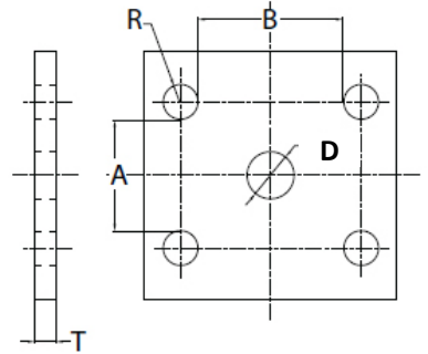
FISHPLATE
