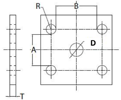
FISHPLATE
