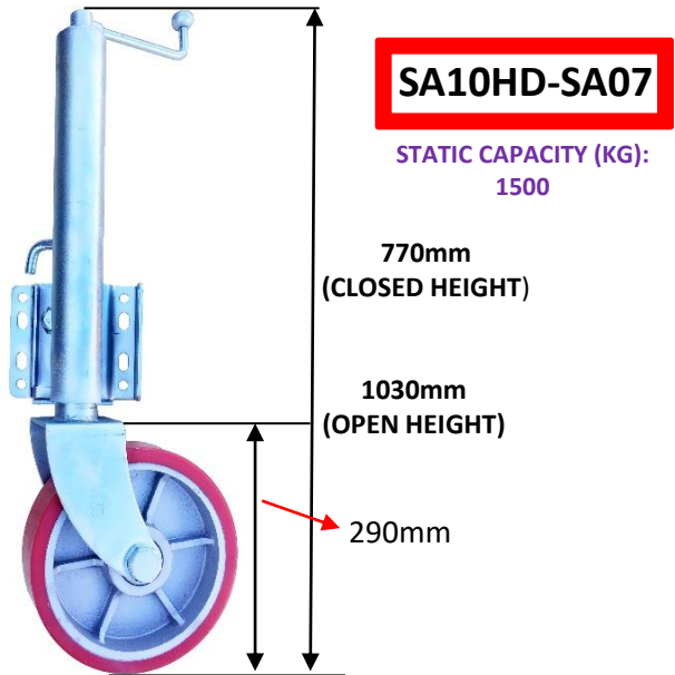
10 x 2 HEAVY DUTY JOCKEY WHEEL c/w SINGLE LOCKING PIN BRACKET
