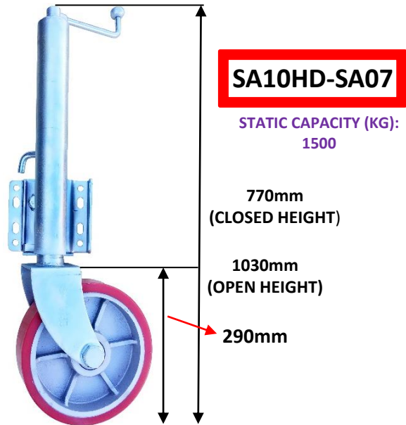
10 x 2 HEAVY DUTY JOCKEY WHEEL c/w SINGLE LOCKING PIN BRACKET
