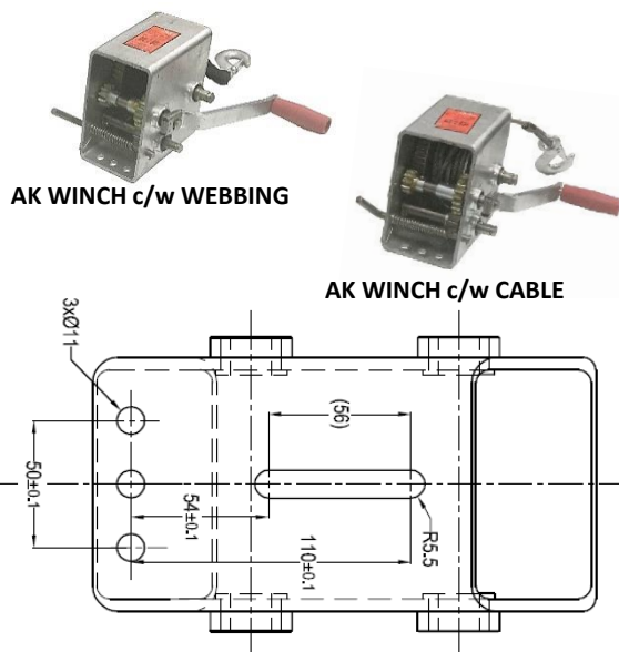
Base/ Mounting Details
