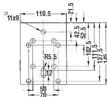
Boltdown Specs.
