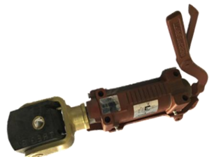
PBMOR POLYBLOCK MECHANICAL OVER-RIDE COUPLING c/w LEVER
