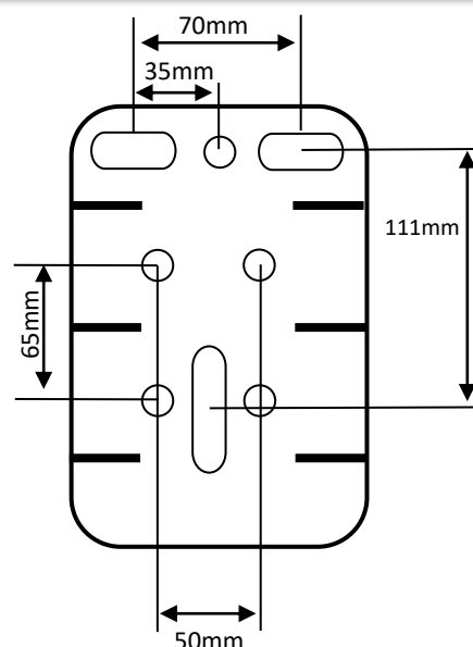
15:1 4.5:1 1:1 BLACK POWDER COATED WINCH c/w 8mtr BLUE WEBBING
