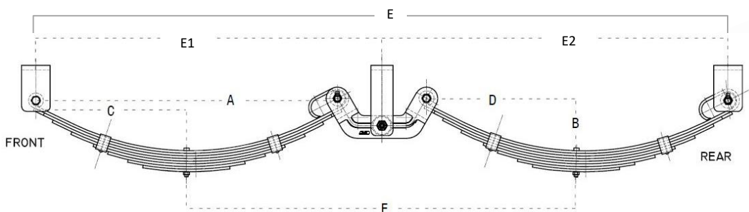
AXLE FITTING
