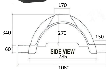
14" PLASTIC MUDGUARDS
