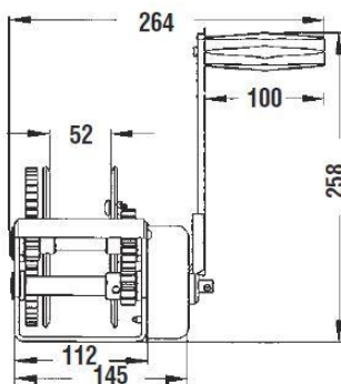
Front Elevation
