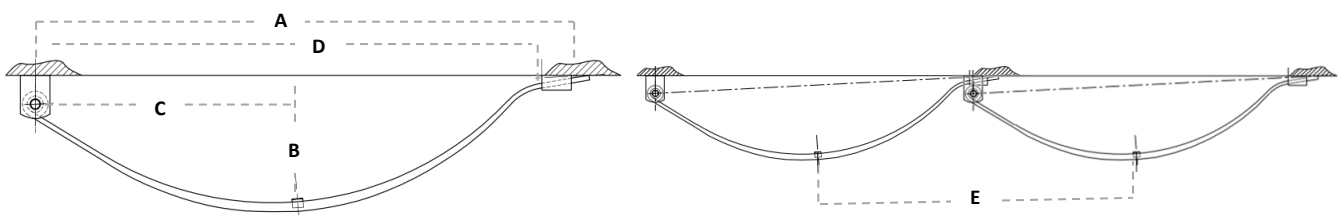
HANGER KIT
