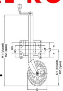
626190 T/T 6 x 2 LIGHT DUTY JOCKEY WHEEL c/w LARGE DOUBLE LOCKING PIN BRACKET
