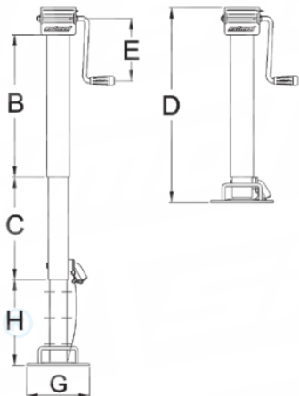
DG590/3SF 70mm Square Side Wind Z/Plated Stand & Bracket (c/w Drop Leg)
