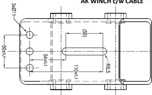
Base/ Mounting Details
