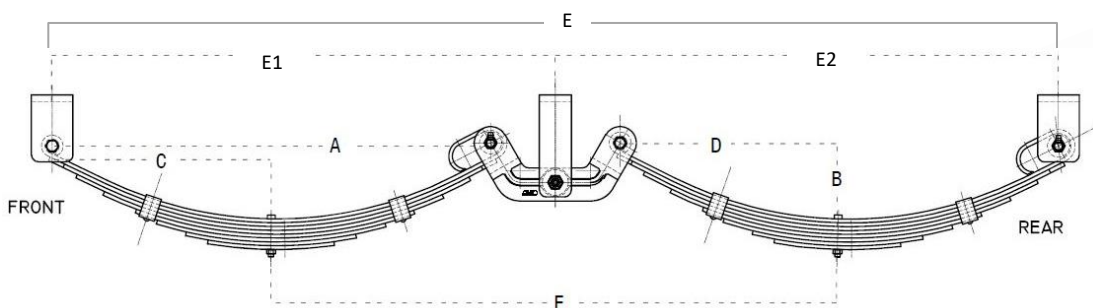
AXLE FITTING
